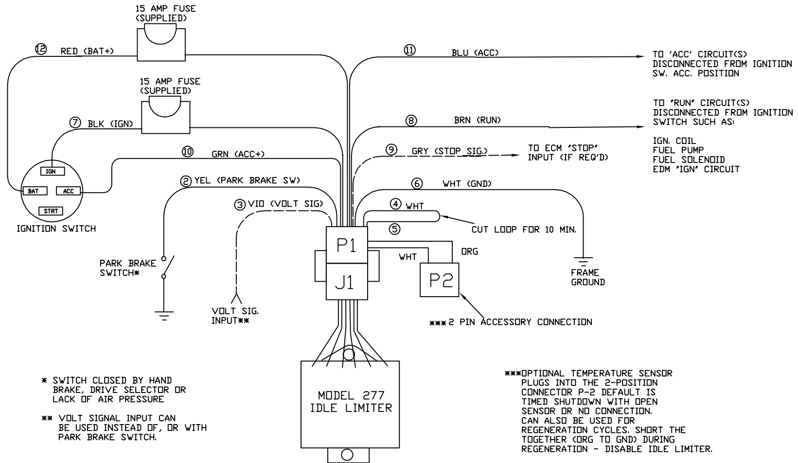
WIRING DIAGRAM MODEL 277 IDLE LIMITER WITH ACCESSORY CONTROL
